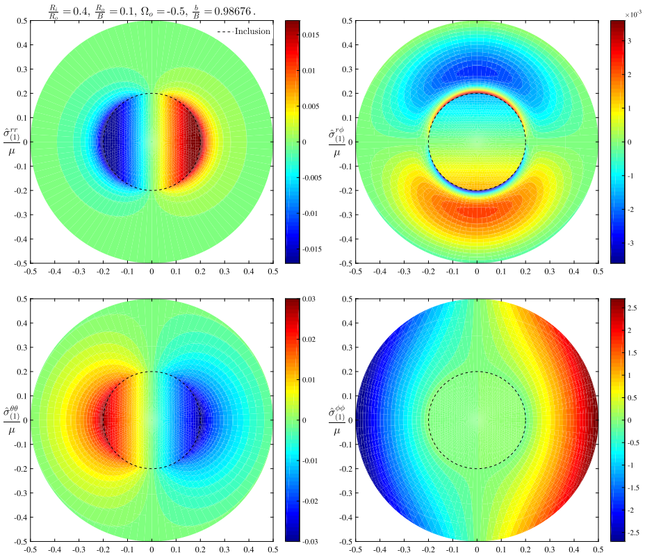
Fig. 5 The first-order physical components of the Cauchy stress in a torus having an inclusion with \frac{R_i}{R_o} = 0.4 , \frac{R_o}{B} = 0.1 , and constant pure dilatational eigenstrain distribution \Omega_o = -0.5 . The ratio of the deformed major radius to the initial major radius of the torus is \frac{b}{B} = 0.98676
