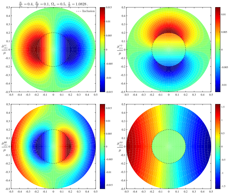
Fig. 6 The first-order physical components of the Cauchy stress in a torus having an inclusion with \frac{R_i}{R_o} = 0.4 , \frac{R_o}{B} = 0.1 , and constant pure dilatational eigenstrain distribution \Omega_o = 0.5 . The ratio of the deformed major radius to the initial major radius of the torus is \frac{b}{B} = 1.0828
