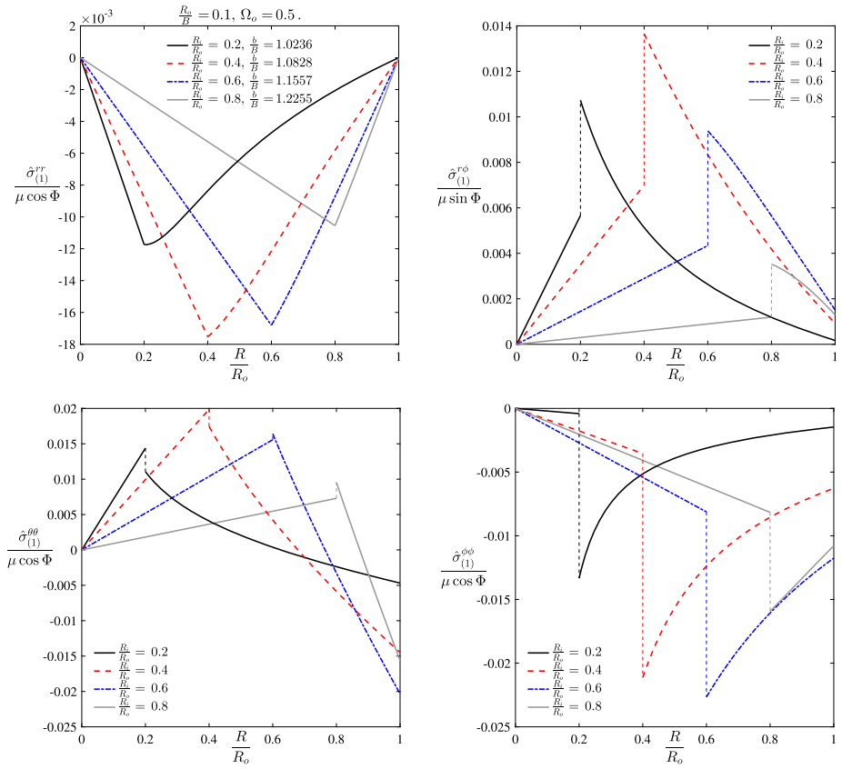
Fig. 3 The radial part of the first-order normalized components of the Cauchy stress tensor for \frac{R_o}{B} = 0.1 , \Omega_o = 0.5 , and different values of \frac{R_i}{R_o}
