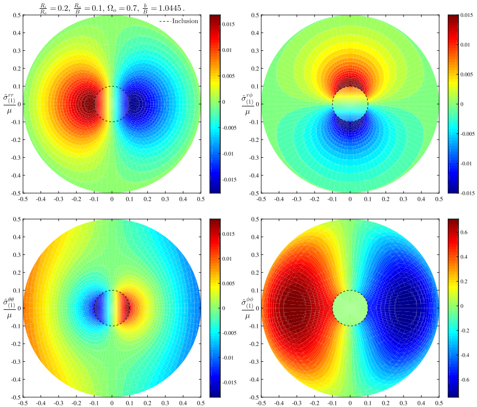
Fig. 7 The first-order physical components of the Cauchy stress in a torus having an inclusion with \frac{R_i}{R_o} = 0.2 , \frac{R_o}{B} = 0.1 , and constant pure dilatational eigenstrain distribution \Omega_o = 0.7 . The ratio of the deformed major radius to the initial major radius of the torus is \frac{b}{B} = 1.0445
