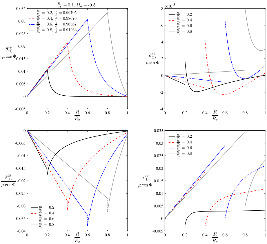
Fig. 4 The radial part of the first-order normalized components of the Cauchy stress tensor for R_o/B = 0.1 , \Omega_o = -0.5 , and different values of R_i/R_o
