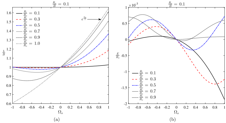
Fig. 8 Variations of \frac{b}{B} and the eccentricity ratio \frac{E}{R_o} as functions of \Omega_o for a torus with \frac{R_o}{B} = 0.1 and different values of \frac{R_i}{R_o} , shown in (a) and (b), respectively
