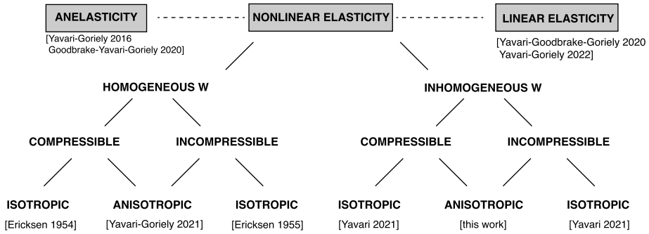
Fig. 1 The universal program: Finding all the universal deformations and displacements, together with the associated universal material preferred directions, and universal inhomogeneities, for both compressible and incompressible solids. These are the different cases considered so far with partial or complete solutions. Here, nonlinear elasticity refers to hyperelasticity and the existence of a strain-energy density W is assumed that can either be homogeneous or non-homogenous, isotropic or anisotropic
